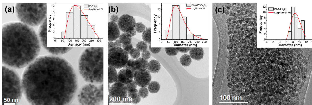
Fig. 1. TEM image of (a) Polystyrene/ \text{Fe}_3\text{O}_4 nanosphere (b) Silica/Polystyrene/ \text{Fe}_3\text{O}_4 nanosphere (c) PAA/ \text{Fe}_3\text{O}_4 nanoparticles.
