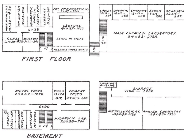
Figure 6. Floor plans to Hanna Hall and the Hanna Chemical Laboratory Annex. North corresponds to the top of the diagram.
