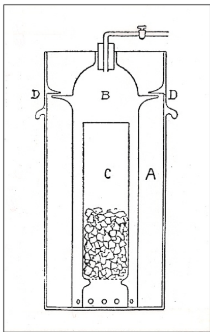
Figure 9. Norton's design for a hydrogen sulfide generator. Made from glazed earthenware, the outer chamber (A) was filled with acid and the inner chamber (C) with iron sulfide. Rotation of the middle chamber (B) until its shoulders (DD) caught on those of the outer chamber, held everything in place. The working principle was the same as that of a Kipp generator and Norton reported that it had "rendered excellent service in the laboratories of the University of Cincinnati."
