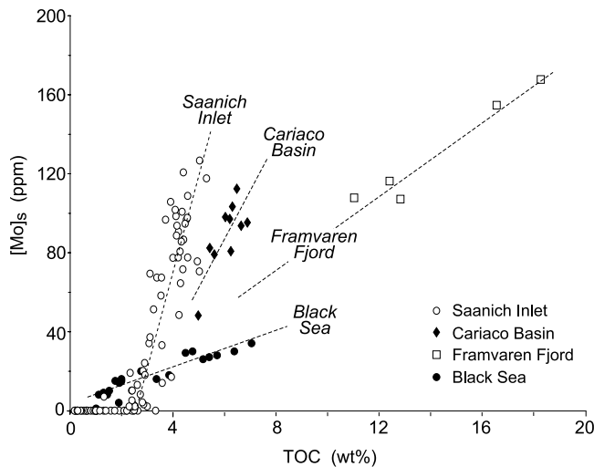
Figure 6. Parsed [Mo]_s -TOC data for modern anoxic silled-basin environments. Regression of the data sets (dashed lines) yields the following slopes ( m , in units of 10^{-4} ): 45 \pm 5 , Saanich Inlet; 25 \pm 5 , Cariaco Basin; 9 \pm 2 , Framvaren Fjord; and 4.5 \pm 1 Black Sea. Data are from sources given in Figure 4.
