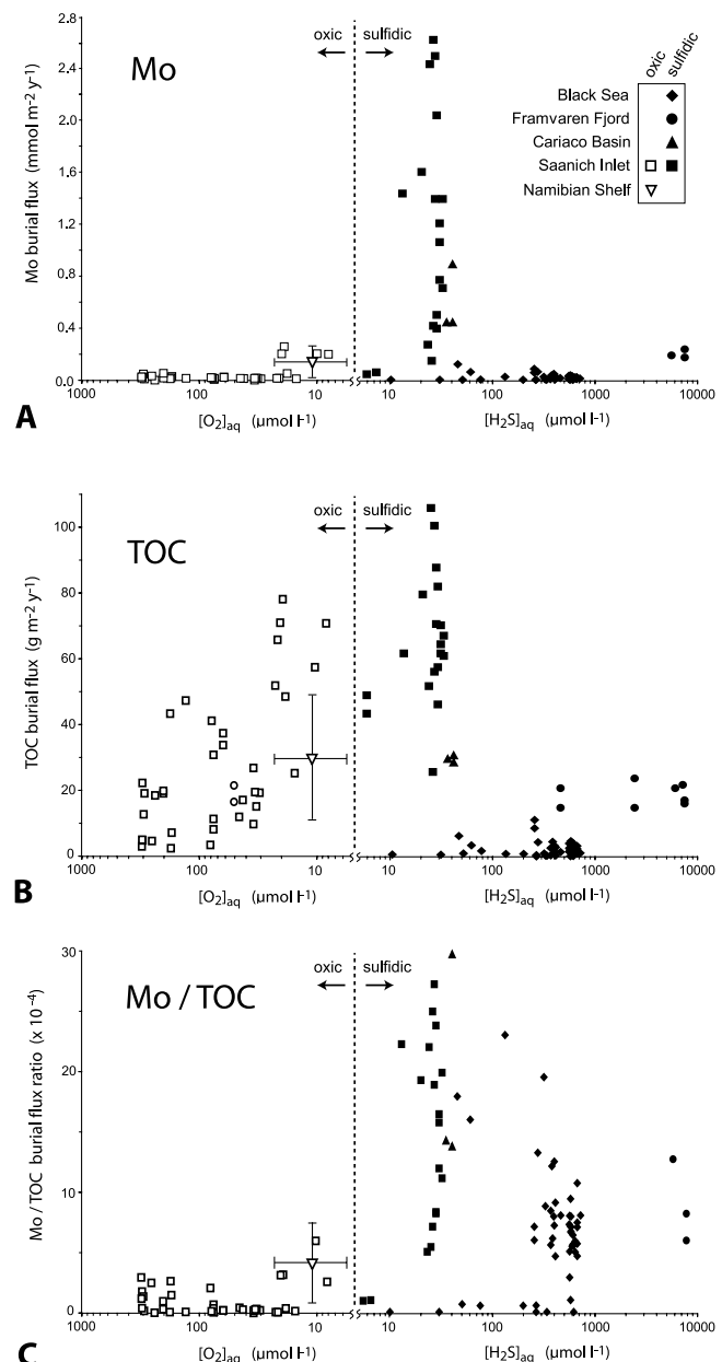
Figure 7. (a) Sedimentary Mo and (b) TOC burial fluxes and (c) Mo/TOC flux ratios versus benthic redox potential for modern anoxic marine environments. Redox potential is represented by logarithmic [O_2]_{aq} and [H_2S]_{aq} scales with more oxic conditions to the left and more sulfidic conditions to the right. Sediment geochemical data are from sources given in Figures 4 and 5, and [O_2]_{aq} - [H_2S]_{aq} estimates are based on sample site water depths from these sources and aqueous chemical data from sources given in Figure 2. Data for the Namibian Shelf are plotted as a mean with a standard deviation cross because no site-specific benthic redox data were available. See text for flux calculations.
