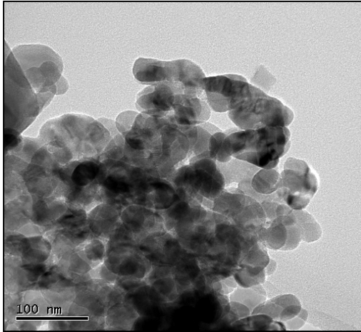
Figure 2 TEM image showing the uncoated ZnO nanoparticles.
