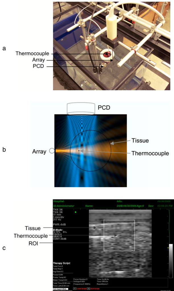
Fig. 1. Experiment configuration. (a) Experimental setup, showing a bovine liver sample with inserted thermocouple, image-ablate array and PCD. (b) Top view showing cross-sectional beam of image-ablate array (horizontal, red) (Mast et al. 2005), cross-sectional sensitivity beam pattern of detector at 1 MHz (vertical, blue) (Mast and Yu 2005) and relative positions of the transducers, thermocouple and tissue. The image-ablate array beam and PCD sensitivity pattern are shown on linear scales, with brightness proportional to amplitude. (c) B-scan of a bovine liver tissue sample from the image-treat array, showing the region-of-interest used for grayscale analysis. The thermocouple tip is seen at the region-of-interest center.
