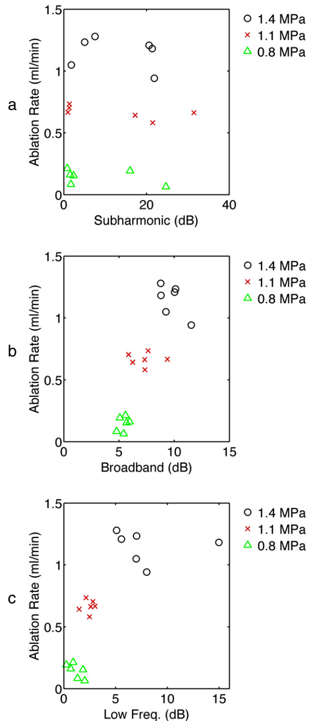
Fig. 6. Scatter plots of ablation rate vs. time-averaged acoustic emission levels for the three frequency bands considered: (a) subharmonic, (b) broadband and (c) low-frequency emissions. Points are shown for all 18 experiments performed at the three exposure conditions used.
