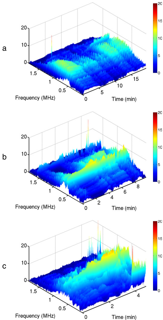
Fig. 3. Time-frequency plots for representative PCD spectra at the three exposure conditions used. Spectra are shown in decibels relative to a measured noise level. All panels show narrow-band subharmonic emissions at 1.55 MHz and broadband emissions throughout the depicted frequency range. Panel (c) also shows low-frequency emissions in the kHz range for times \geq 4 min. (a) 0.8-MPa nominal sonication amplitude. (b) 1.1 MPa. (c) 1.4 MPa.
