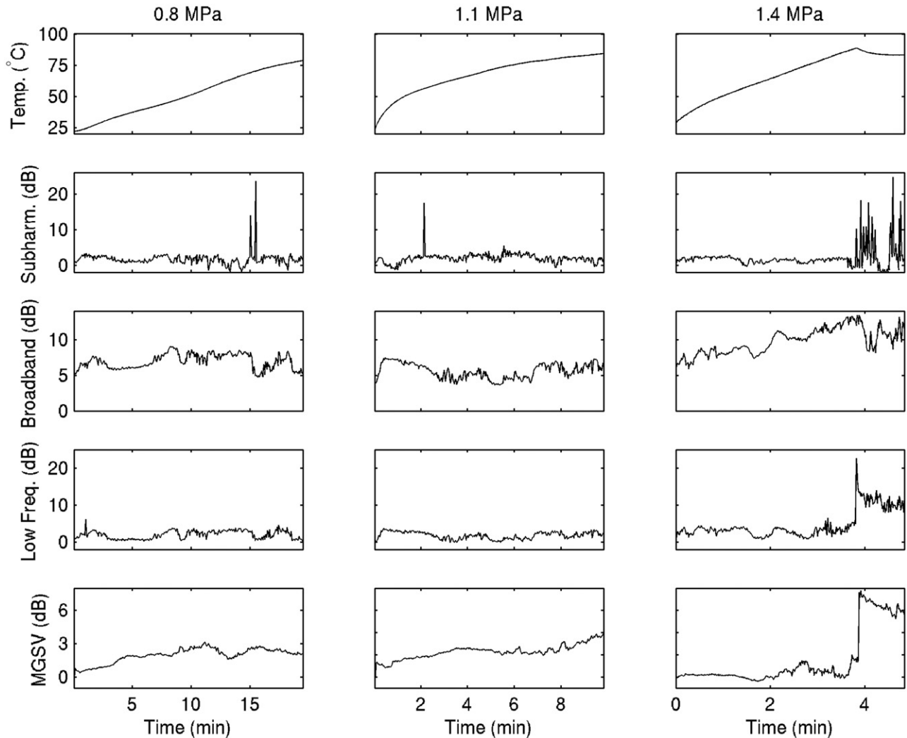
Fig. 5. Representative plots of the measured time-dependent temperature, acoustic emission levels and B-scan mean grayscale value for one ablation experiment at each of the three exposure conditions used.
