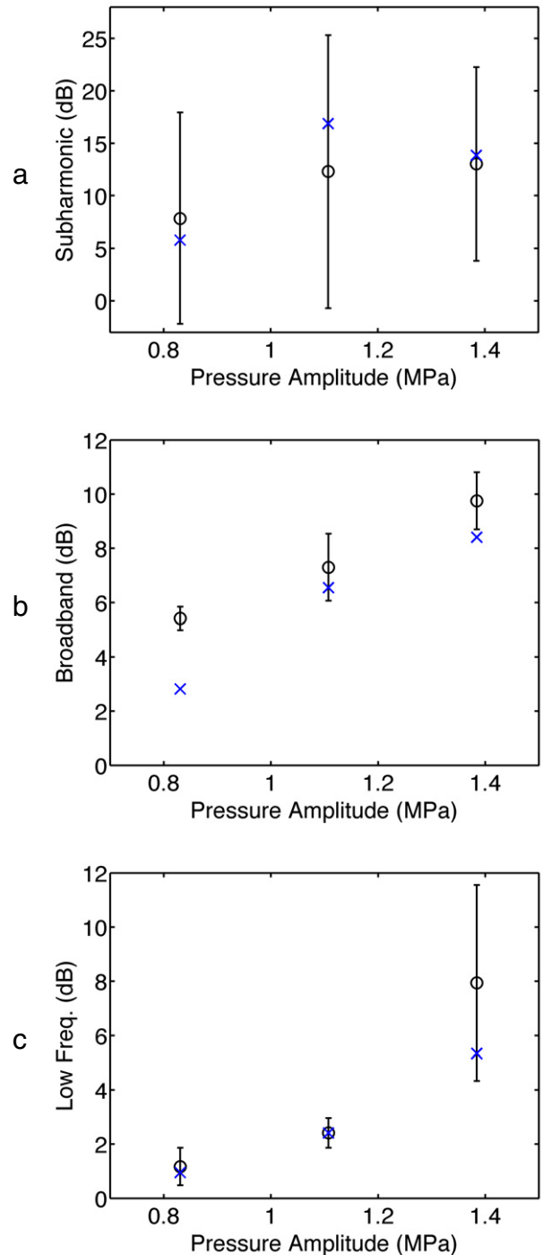
Fig. 4. Average levels for PCD-measured acoustic emissions within subharmonic, broadband and low-frequency intervals at the three exposure conditions used. Plotted as circles with error bars are the mean and standard deviation of the average emission level for each pressure amplitude ( N = 6 for each). The plotted "x" symbols show average acoustic emission levels in each band for two experiments without the needle thermocouple at each exposure condition.
