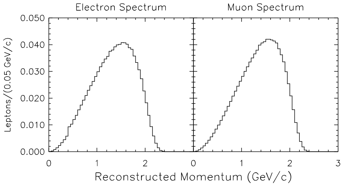
Figure B.2: Reconstructed momentum spectra for electron and muons in the ISGW model with 21% D^{**} .
