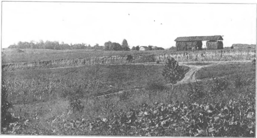
B.—The surface silt being stripped from uplands near Delhi, O., to be used for cupola lining. (See p. 180.)
