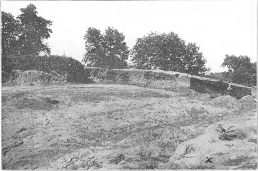
A.—Loess being stripped from hilltop at Bellevue, Ky., for molders' sand. (See p. 182.)
