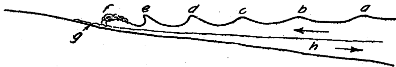
Fig. 14.—Diagram showing incoming breakers and outgoing undertow. Arrows show the movement of the water. a, b, c, d, e —waves advancing on shore, becoming shorter, higher, and steeper on front. f —breaker; g —out-rushing water of the last breaker; h —undertow.
