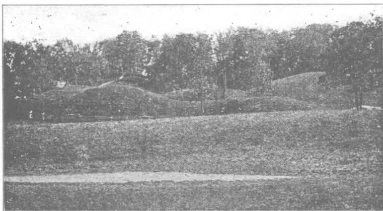
Fig. 46.—Kames near Oconomowoc, Wis. Similar topography is found in the kame districts around Camp Hageman and Furmandale.
