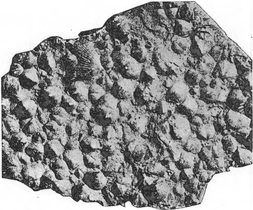
Fig. 28.—Fossiliferous limestone, Dalmanella Zone , near top of Eden group. (Chamberlin and Salisbury).
