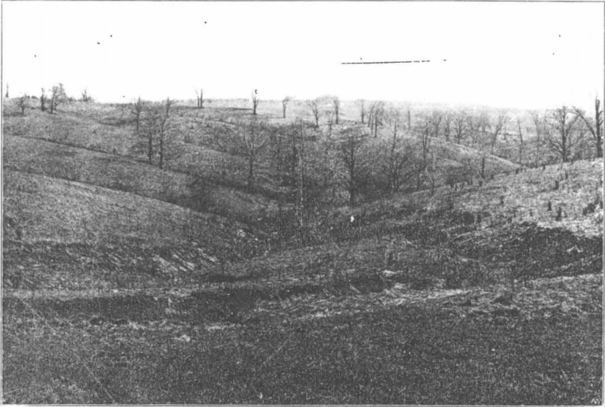
A.—Reviled valleys in upland, West Covington, Ky., city park tract.
