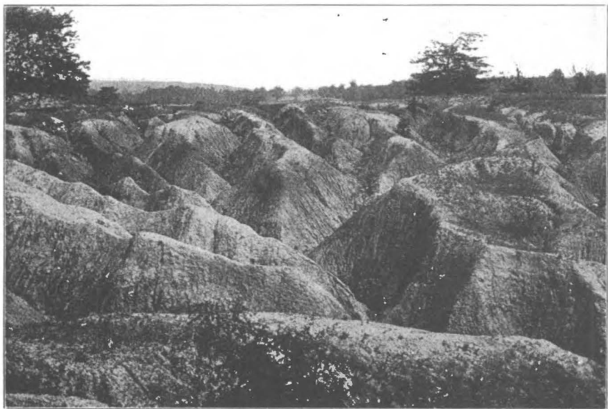
B.—Badlands eroded from the older glacial drift, west of Spring Grove Cemetery, Cincinnati. (Compare figures, pp. 86-88.)
