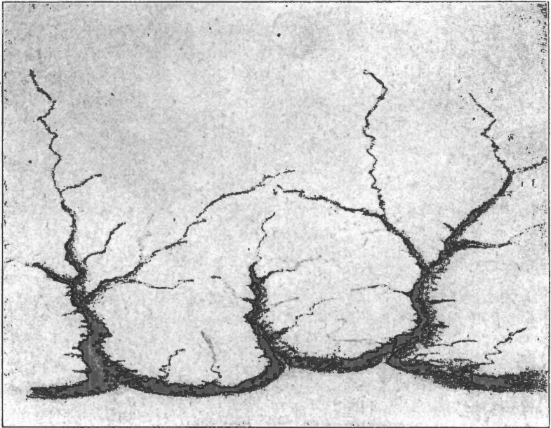
Fig. 32a.—The deepening, widening, and lengthening of valleys. This figure represents an early stage; compare figs. 32b, p. 87, and 32c, p. 88. (Salisbury and Atwood.)
