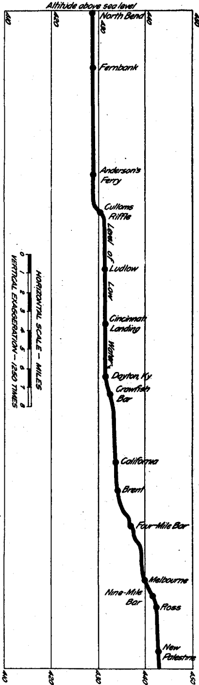
Fig. 5.—Profile of Ohio River from New Palestine to North Bend.
