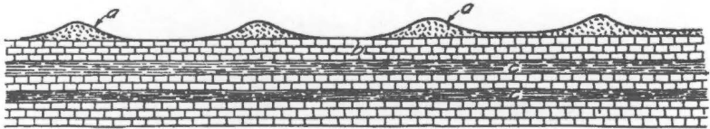
Fig. 19.—Diagram of large ripple marks on limestone, two to three feet from crest to crest. a —fragments of shells, etc., not much worn by water; locally (at the right) continuous from crest to crest; elsewhere absent between ridges; b —dense blue limestone; c —shale.
