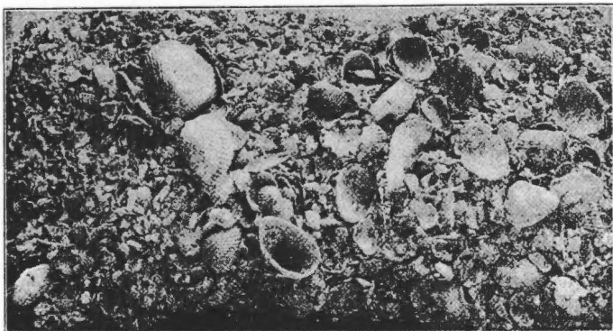
Fig. 16.—Modern shell limestone; coquina from Florida. (Scott's Introduction to Geology.)
