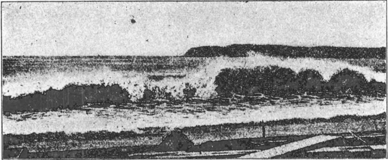
Fig. 13.—Breaking waves (Maury-Simonds).
