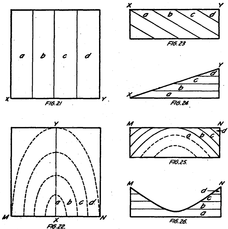
Figs. 21-26. —Diagrams to illustrate the nature of geologic maps. Fig. 21 represents a geologic map in which (a) is the lowest and oldest bed and (d) the youngest. Figs. 23 and 24 are two cross sections, either of which is consistent with this map. Fig. 22 is also a geologic map in which (a) is the lowest and (d) the highest bed. Its cross section along the line MN may be either as shown in Fig. 25 or as in Fig. 26. In the former case its section along XY will be as in Fig. 23; in the latter case as in Fig. 24.
