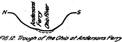
FIG. 12. Trough of the Ohio at Andersons Ferry
