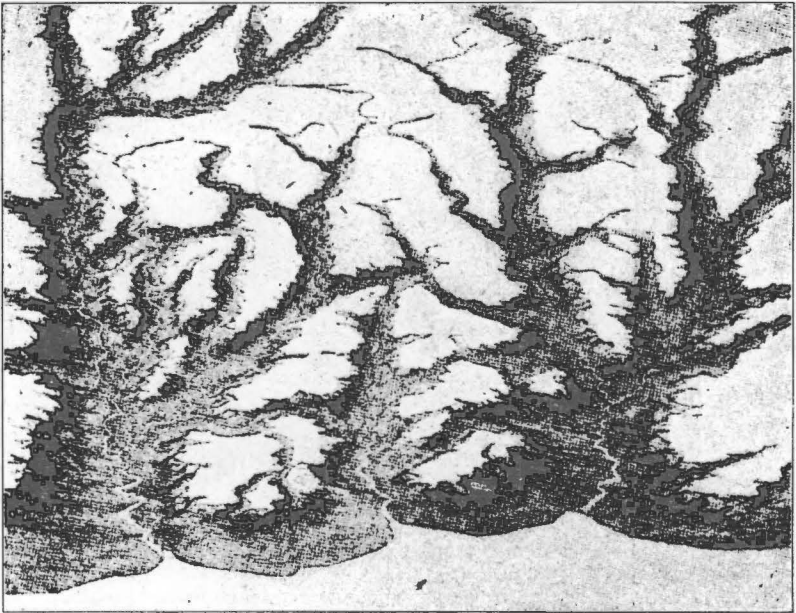
Fig. 32c.—A still later stage in the deepening, widening and lengthening of valleys (Salisbury and Atwood.)
