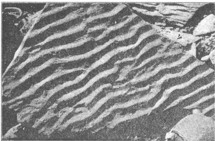
Fig. 17.—Ripple-marked sandstone (Fairbanks).
