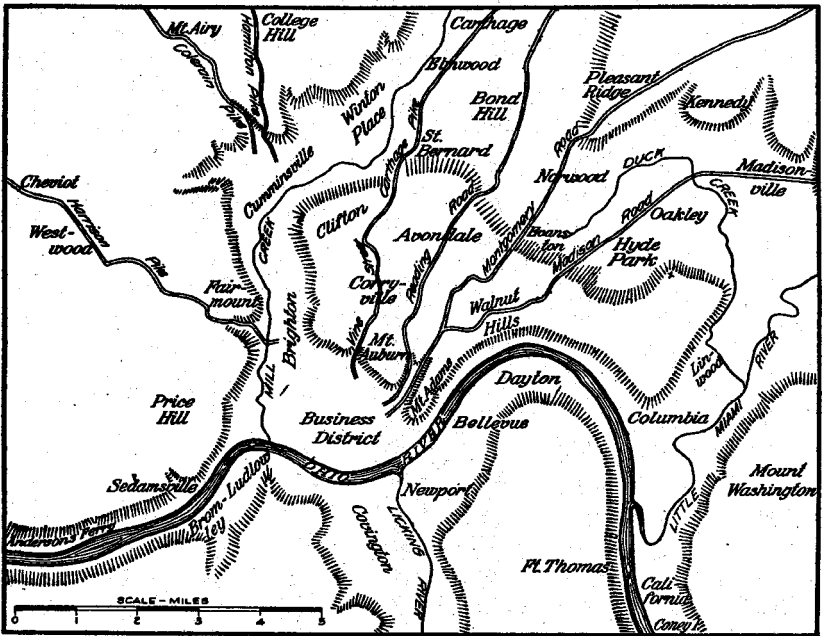
Fig. 59.—The site of Cincinnati.
