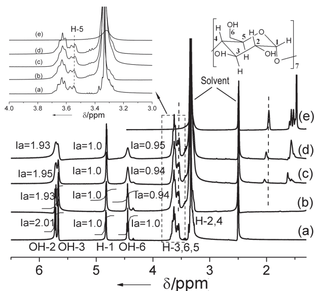
Figure 4. ^1\text{H} NMR spectra of \beta -CD (a), freeze-dried GNS/ \beta -CD (b), freeze-dried GNS/ \beta -CD/Ad-NH _2 with increasing loading ratio of Ad-NH _2 [(c) 3.88 wt%, (d) 5.71 wt%] and Ad-NH _2 (e). (DMSO- d_6 as solvent, "Ia" denotes integrated area)
