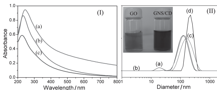
Figure 2. (I) UV-vis absorption spectra of GO dispersion (c) and after reduction with ammonia and \beta -cyclodextrin at 80 °C for 2 h (a) and 1 h (b), respectively. (II) Size of GO (a); GNS/ \beta -CD (b) and GNS/ \beta -CD stored at room temperature for one month (c) and three months (d). Inset shows the color change of 0.05 mg mL -1 GO solution before and after reduction.
