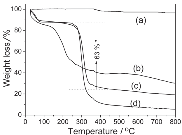
Figure 7. TGA curves of flake graphite (a), GO (b), GNS/ \beta -CD hybrid (c), and \beta -CD (d) obtained under a nitrogen flow of 100 \text{ mL min}^{-1} with the heating rate of 5 \text{ }^\circ\text{C min}^{-1} .
